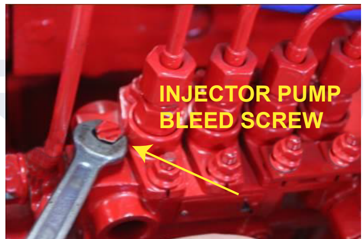
FIGURE 21 - INJECTOR PUMP ASSEMBLY BLEED SCREW
