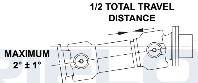
FIGURE 5 - DIESEL ENGINE OFFSET ANGLE & SPACING
