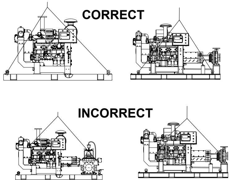
FIGURE 1 - PROPER LIFTING
