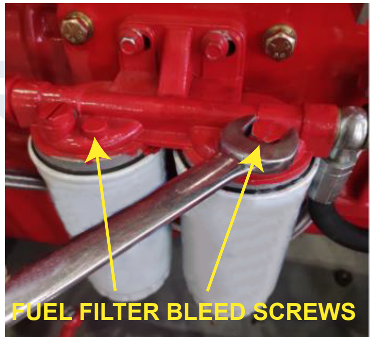
FIGURE 21 - FUEL FILTER BLEED SCREWS
